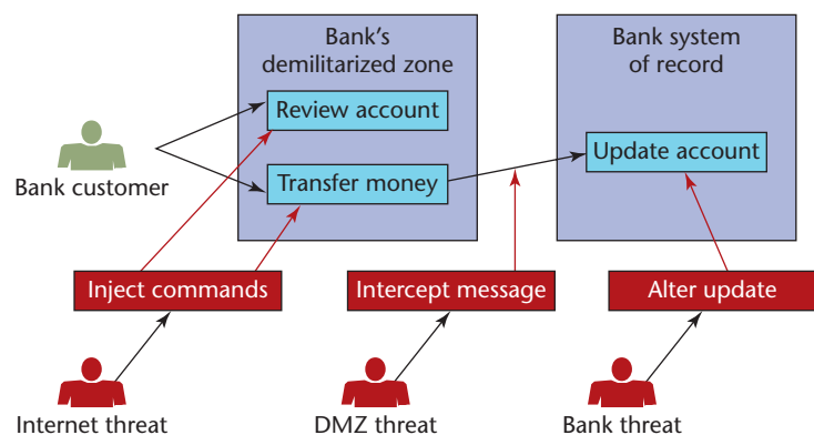
Figure 2. Misuse case. Using the same scenario as in Figure 1, we can see how attackers might approach the bank customer’s account.
